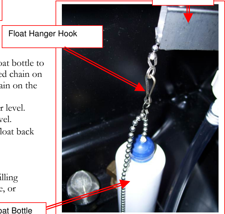
Float Valve
